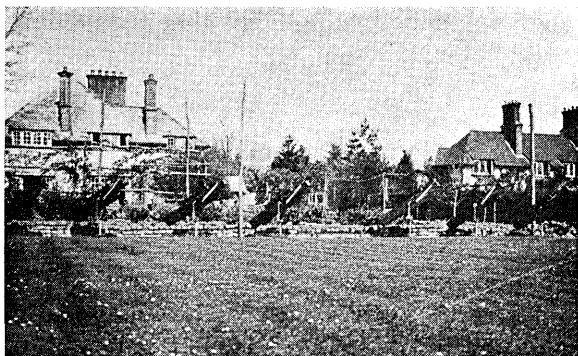
Fig. 5. Comparison of Féry spectrographs at Boar's Hill, Oxford, 1926.
